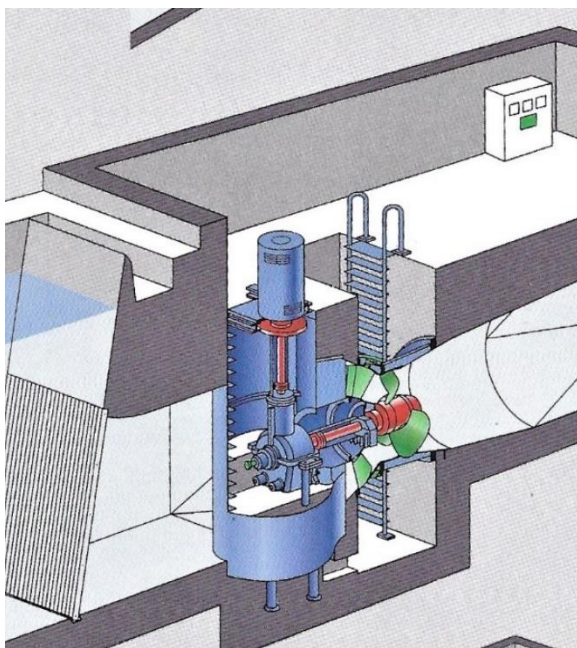
Figure 47: Tubular pit turbine with a bevel speed increaser (Voith, 1990s)
