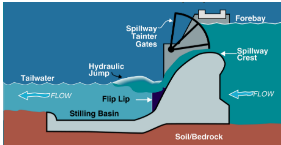
Figure 63: Segment (Tainter) gate (USACE, n.d.)
