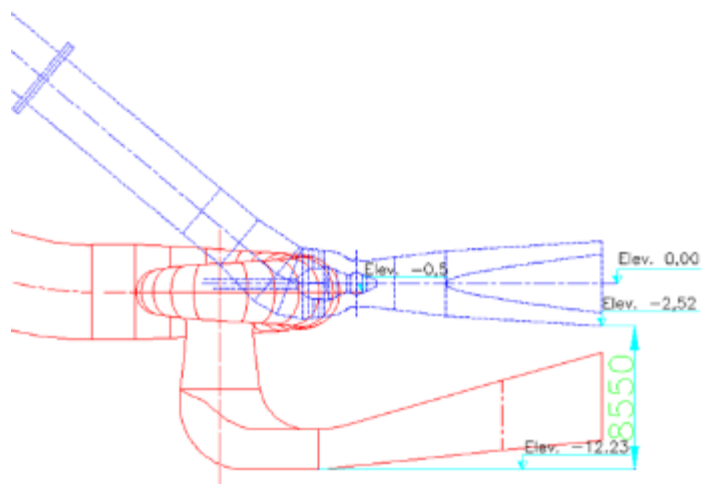
Figure 27: Comparison between excavation work needed for classic Kaplan turbines (2 units) and 4 tubular SAM turbines (4 units) with the same total capacity (Czerwinski, Canas, and Marin, 2012)
