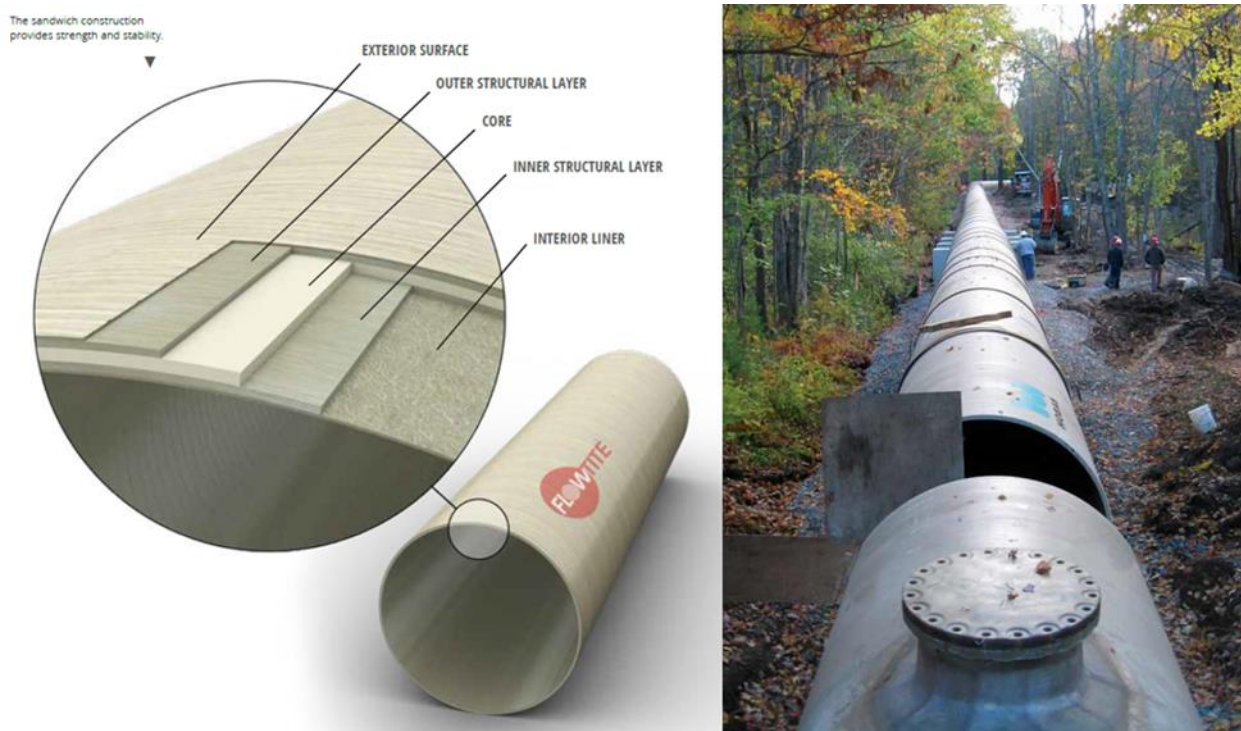
Figure 73: Flowtite pipe structure (left) and replacement of a wood stave penstock segment by a Hobas GRP pipeline (right). Jackman Hydro Station, Hills-borough, New Hampshire, USA (Amiblu, 2020)
