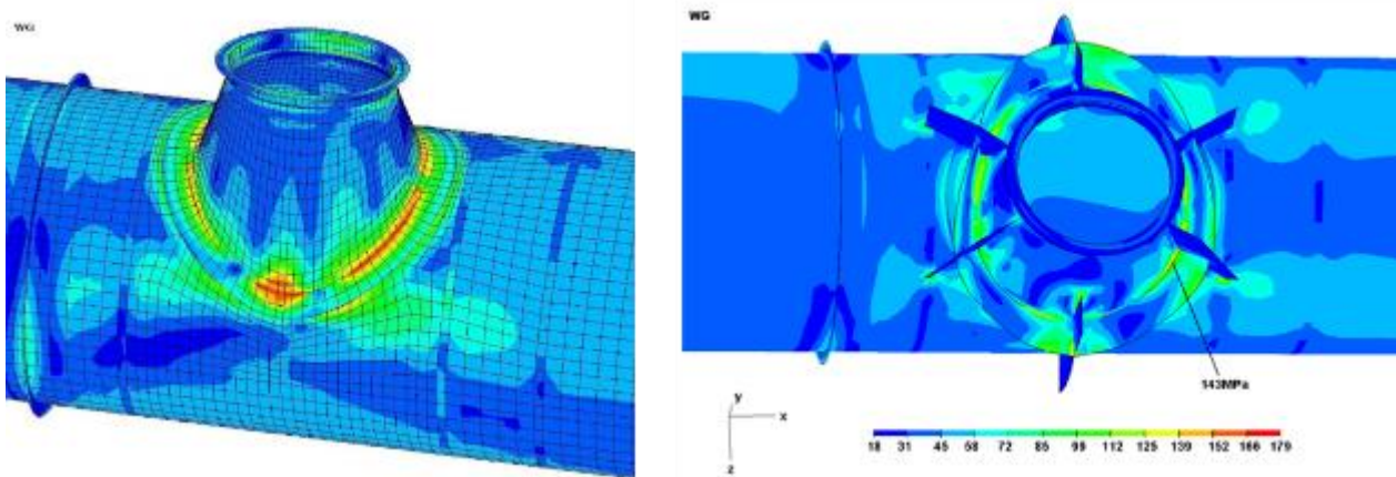
Figure 70: Tensile effort (MN/m 2 ) distribution at penstock branching node (Adamkowski et al, 2019)
