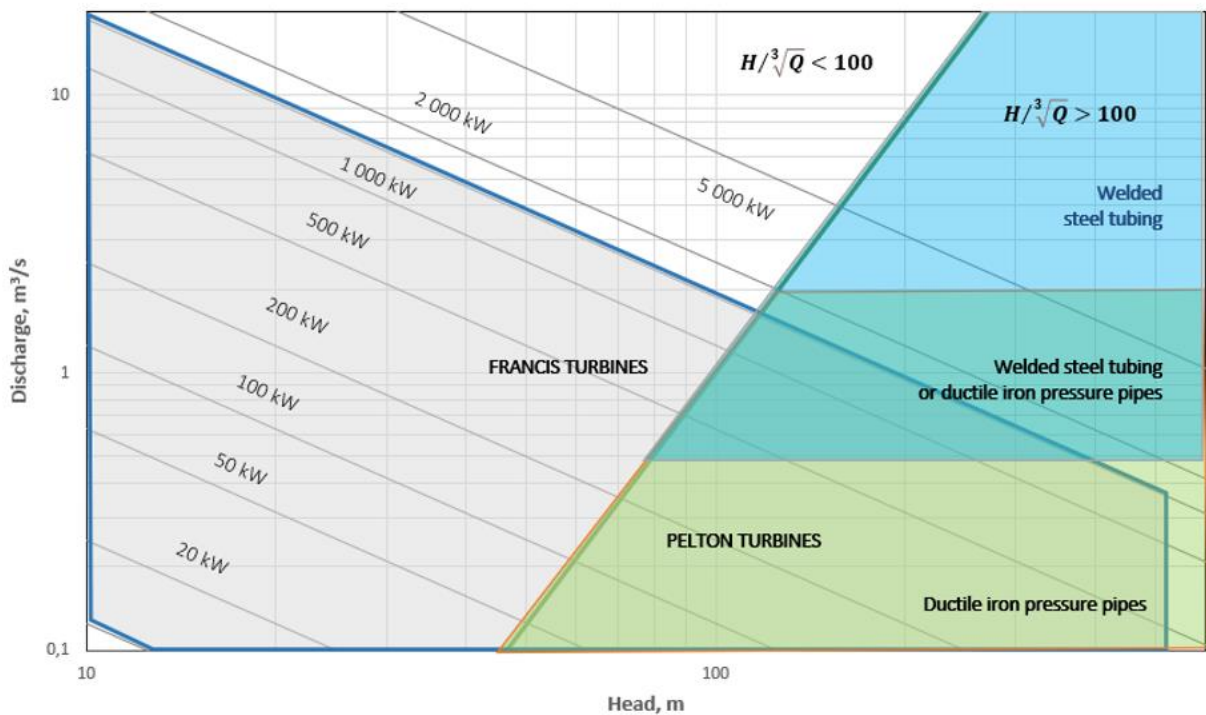
Figure 71: Typical steel and ductile iron penstock small hydro application ranges (Steller, 2020 after anon)
