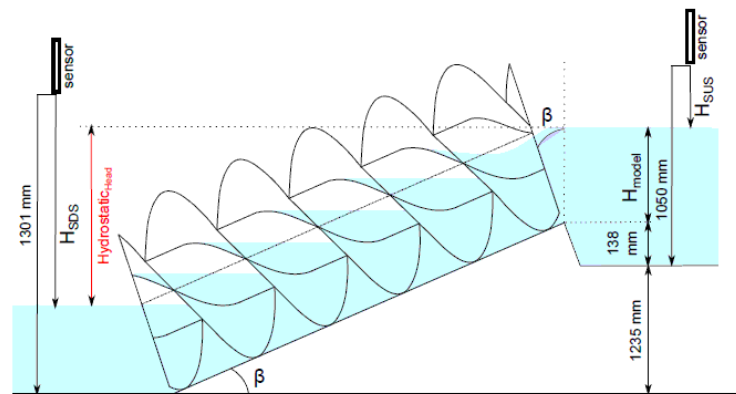
Figure 44: Schematic view of an Archimedes screw runner showing instantaneous positioning of water in "buckets" formed by the screw blading (Rohmer et al., 2016)
