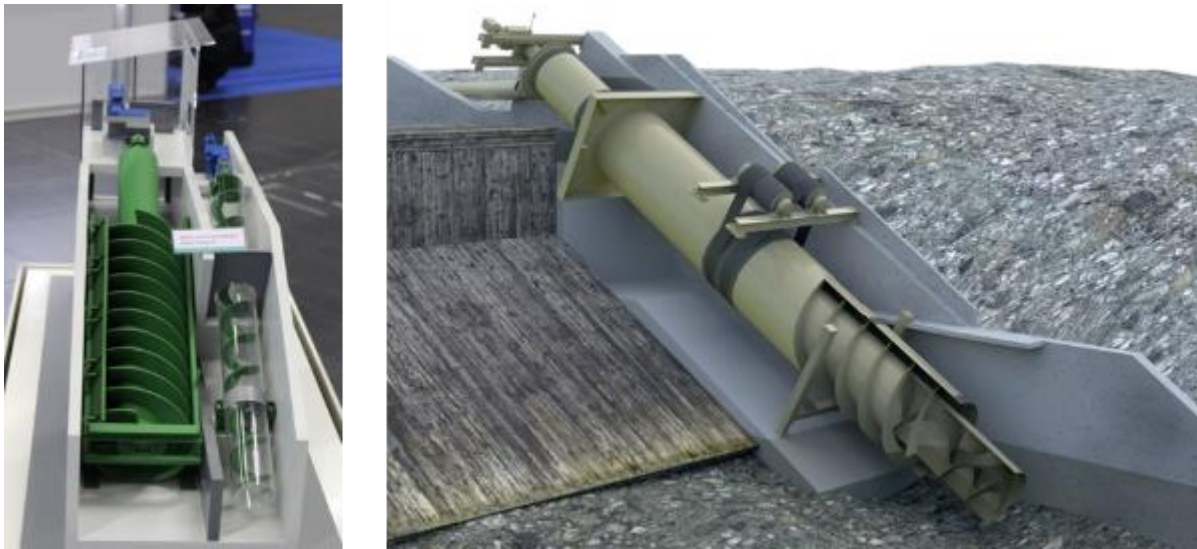
Figure 45: A parallel Archimedes screw set by Rehart Power (left) and a 3D view of Hydroconnect coaxial screw unit (right) at the RENEXPO Interhydro Fair in 2017 (source: J. Steller)
