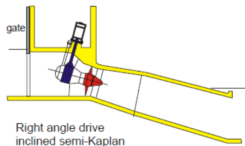
Figure 29: A compact semi-Kaplan unit with bevel speed increaser (ESHA, 2004)
