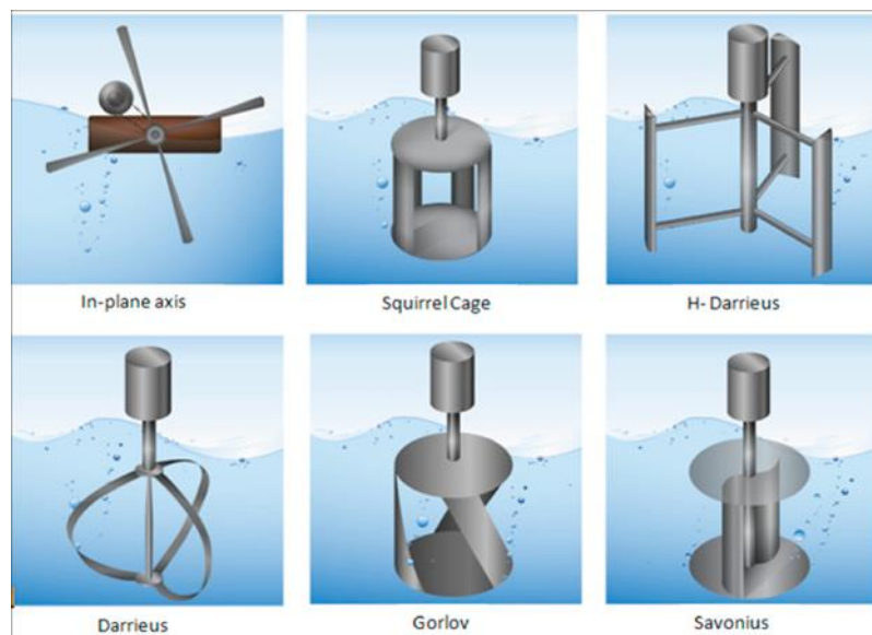
Figure 40: Vertical axis kinetic turbine (Khan, 2009)
