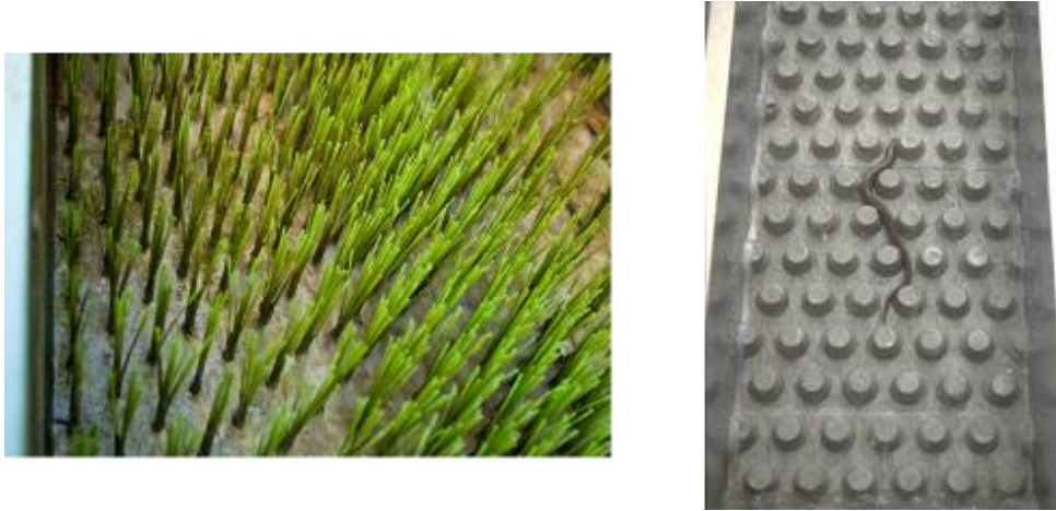
Figure 79: Eel ramp covered by a brush type substrate (left) and (right) a concrete cones substrate (source: AFB)
