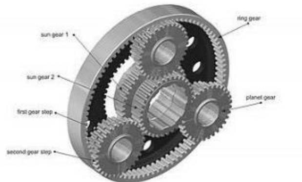
Figure 51: A double sun planet gear as offered by Rohloff AG (2020)
