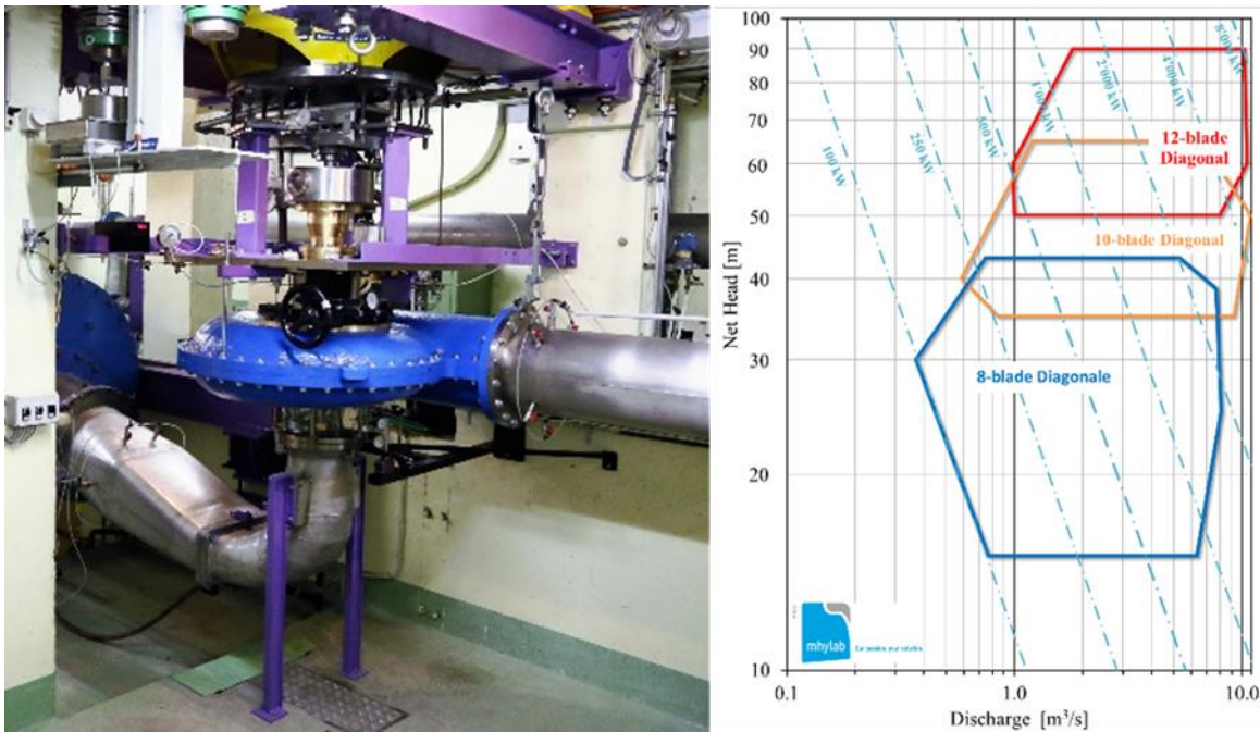
Figure 34: The Mhylab diagonal turbine (Bullani and Denis, 2019)
